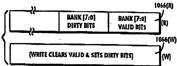
Fig. 37H BANK STATUS REG
